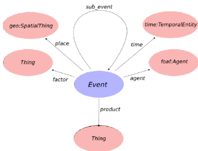
Fig. 4 Event ontology [29]
