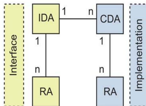
Fig. 5 JXTA advertisements
