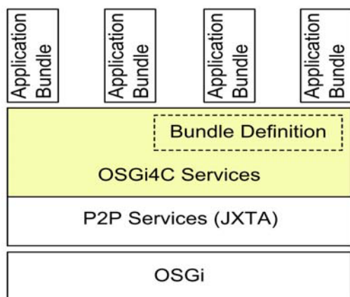
Fig. 3 OSGi4C Architecture
