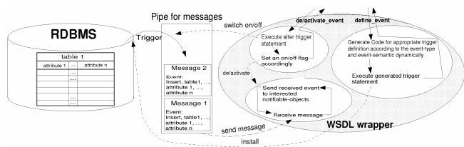
Fig. 2 Monitoring: Triggers and Callbacks
