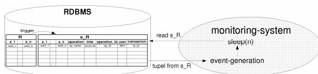
Fig. 3 Monitoring: Triggers and Polling
