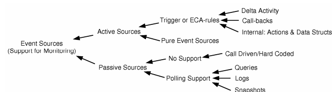
Fig. 1 Classification: Monitoring Support
