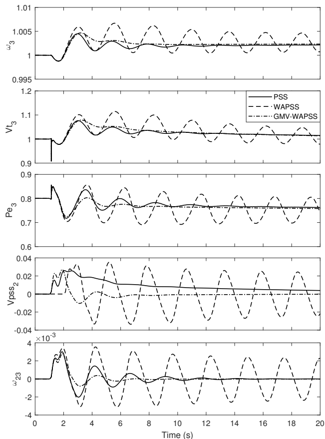
Fig. 4. Step of 5% at the reference voltage of generator 1.
